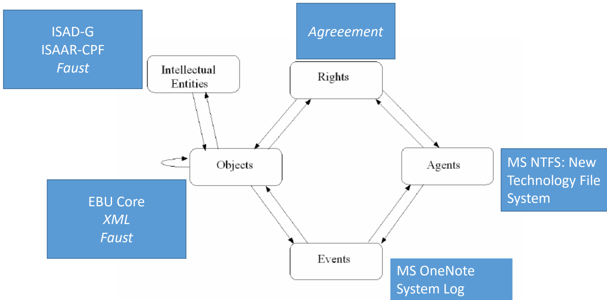
Figure 1: The PREMIS Data Model
